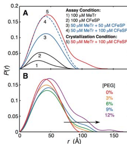
Figure 10. Pair-distance distribution, P(r) , plots of species in CFeSP/MeTr mixtures. (A) Under assay conditions, the maximum particle dimensions, D_{\text{max}} for the free subunits are <100 Å and consistent with the crystal structures of the individual proteins. 9,11 D_{\text{max}} values for CFeSP/MeTr mixtures also do not exceed 100 Å under assay conditions (blue curves), while D_{\text{max}} extends to \sim 140 Å under crystallization conditions (red curve). This result is consistent with the 1:1 CFeSP/MeTr complex being the largest species under assay conditions, even in the presence of excess CFeSP (blue dashed curve), and the appearance of the 2:1 CFeSP/MeTr complex under crystallization conditions. (B) Titration of PEG MME 5000 into a solution with 100 \mu\text{M} CFeSP and 50 \mu\text{M} MeTr leads to an increase in D_{\text{max}} from \sim 100 Å toward \sim 140 Å. At the maximum PEG concentration tested, 12%, even higher order oligomerization is detected ( D_{\text{max}} > 150 Å). For comparison, the PEG MME 5000 concentration is 3% in the crystallization condition.
